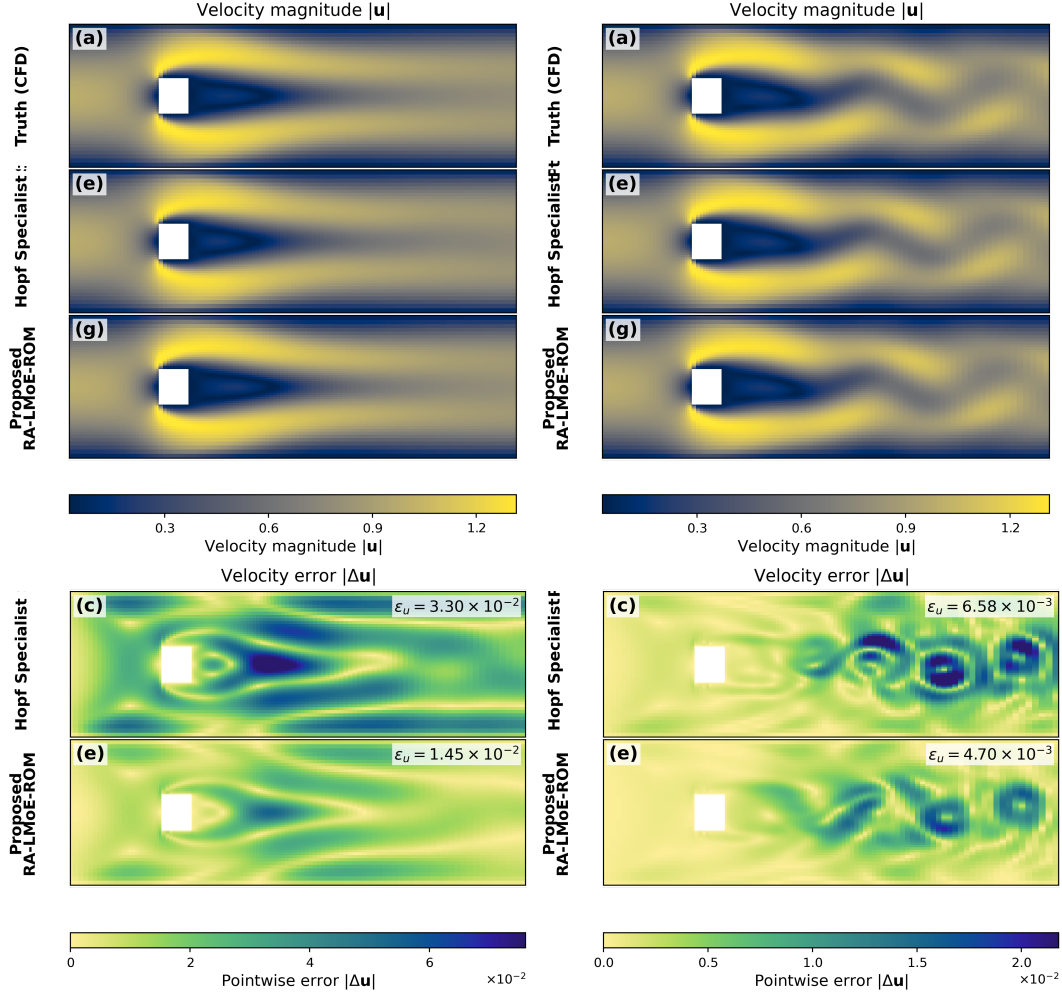
Figure 2: Representative centered-square overlap predictions for S-H (left) and H-P (right). T2-C combines independently evolved local predictions only after reconstruction in physical space. The displayed examples illustrate the corresponding reduction in velocity-field error; complete velocity and pressure comparisons are reported in Appendix G.
